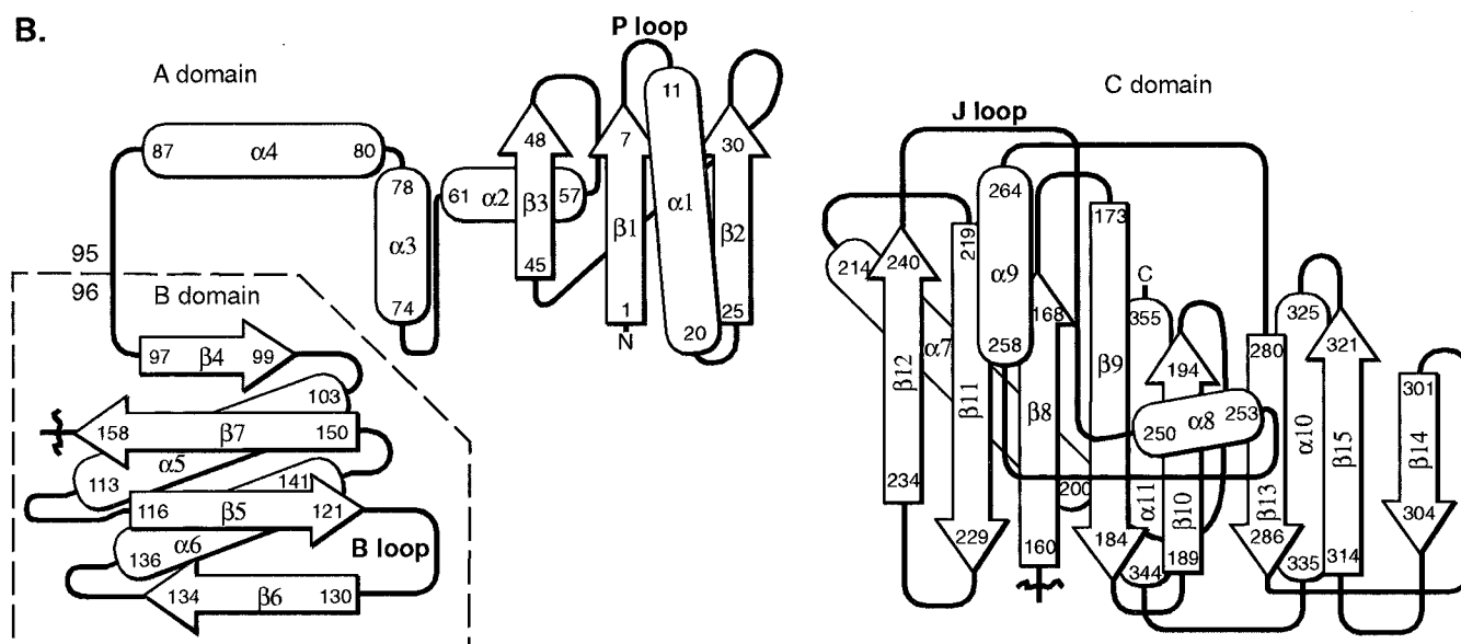
FIGURE 4: Secondary structure and strictly conserved amino acid residues in PurKs. (A) Sequence of E. coli PurK. The white letters in black boxes are conserved among 22 full-length PurK sequences. Black letters in white boxes are conserved among 21 PurK sequences. Triangles indicate where any insertion is required in the E. coli sequence to generate the indicated consensus sequence. (B) Topology diagram of the secondary structure of the A, B, and C domains of PurK. For clarity, the linker between β7 and β8 is not shown, and the C domain has been moved to the right of the A and B domains.
